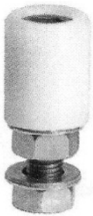
60.040 Ø 25 mm 0,118 kg 60.040.01 Ø 31 mm 0,128 kg 60.040.02 Ø 33 mm 0,135 kg 60.040.03 Ø 36 mm 0,141 kg 60.040.05 Ø 41 mm 0,153 kg
