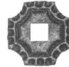
13.316.20 H 75 x L 75 mm □ 20,5 mm gr. 5 mm 0,150 kg
