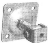
15.250.07/20 □ 97 x 97 mm gr. 5 mm M 20 0,750 kg
